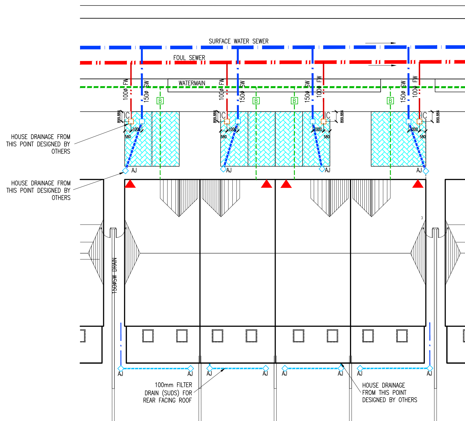
TYPICAL HOUSE CONNECTIONS LAYOUT SCALE 1:200
